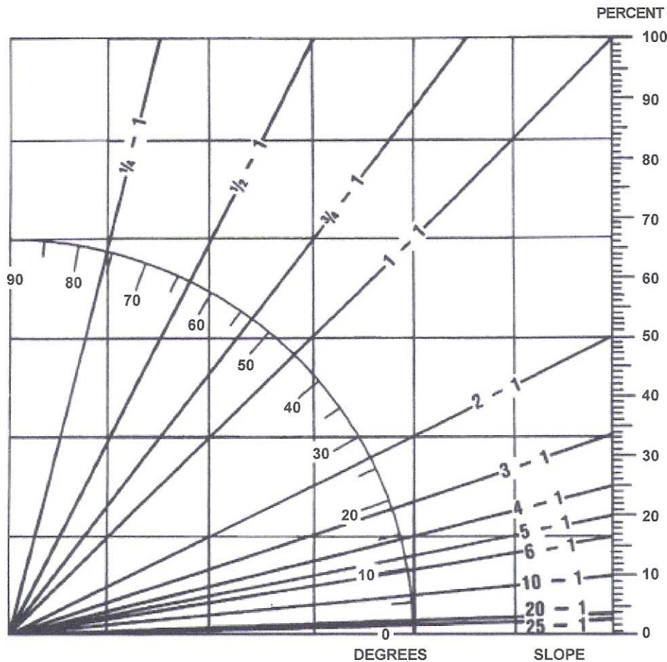
GRADE COMPARISON CHART DEGREES - PERCENT - SLOPE
